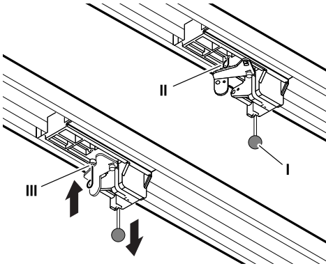
Fig. 8: Disengaging and engaging the drive
