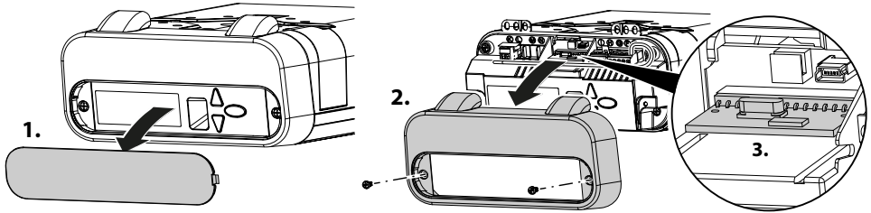
Fig. 2: Opening the cover on the drive head and determining the radio module type
