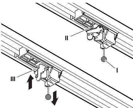
Fig. 18: Disengaging and engaging the drive
